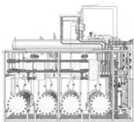
4 cell stacks = 70 Nm 3 /h
