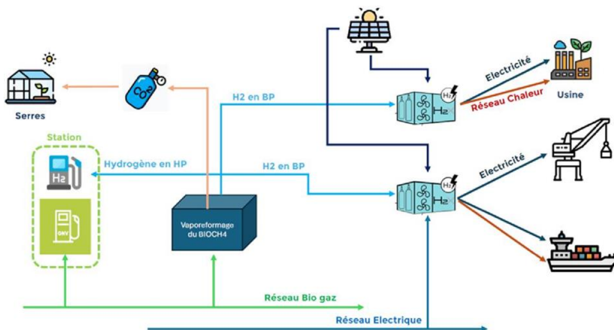
Figure 5: Small-scale hydrogen production system (source :Port of Brest)
