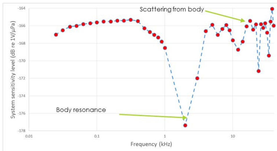
Figure 2. Example of the frequency response of a recorder with hydrophone fixed rigidly to the body.
