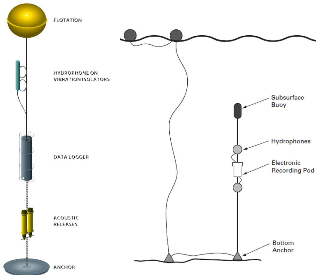
Figure 3 Examples of the bottom-mounted autonomous recorder deployment configurations.
