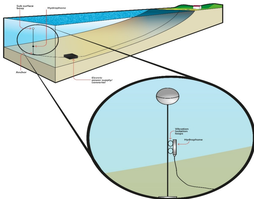
Figure 4 The Bottom-mounted hard-cabled to shore deployment option.
